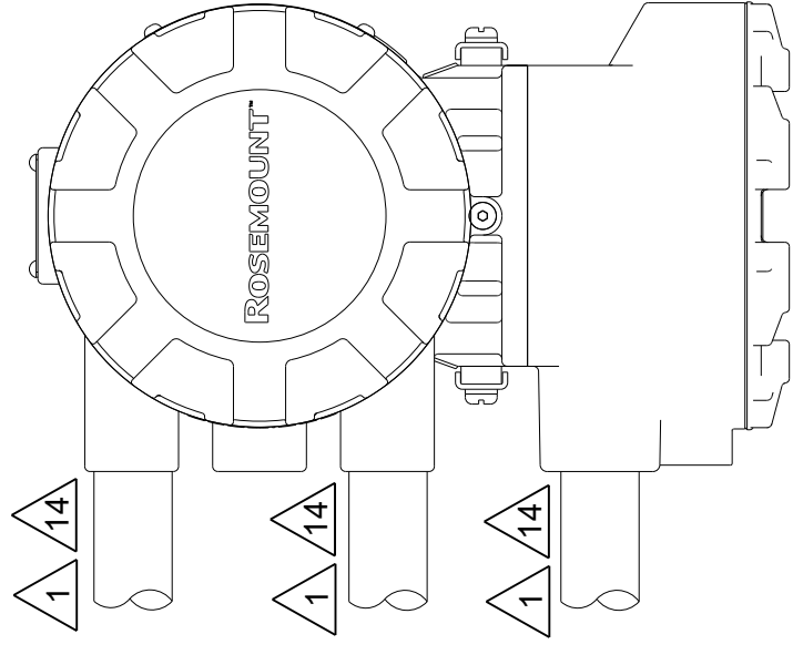
MODEL 8750WDMR REMOTE MOUNT ZC OPTION
