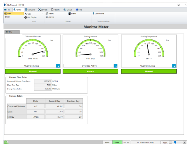
Monitor Screen
