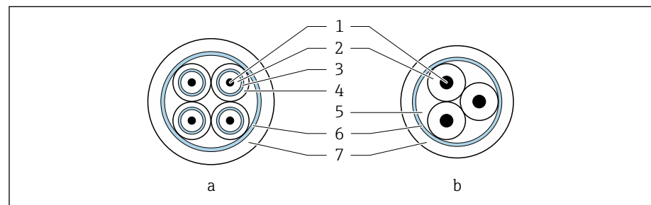
3 Cable cross-section
