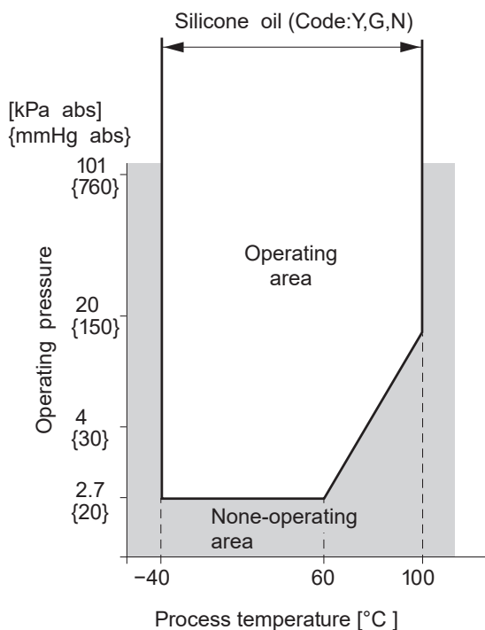
Fig. 1 Relation between process temperature and operating pressure
